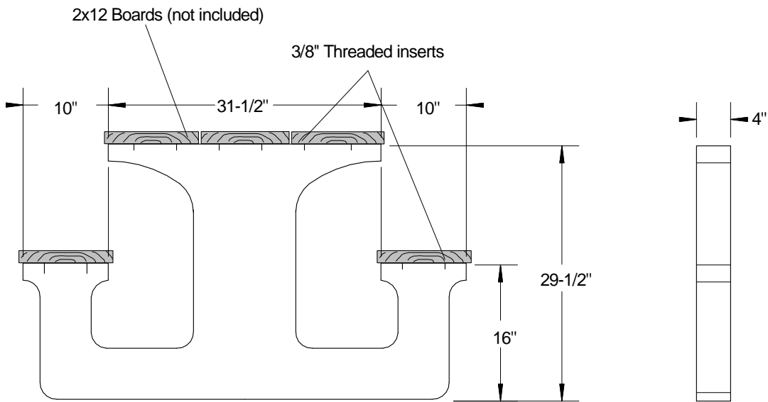
End View
