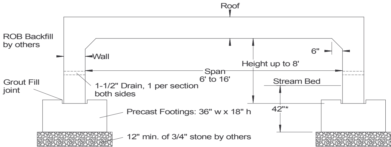
Side Elevation
