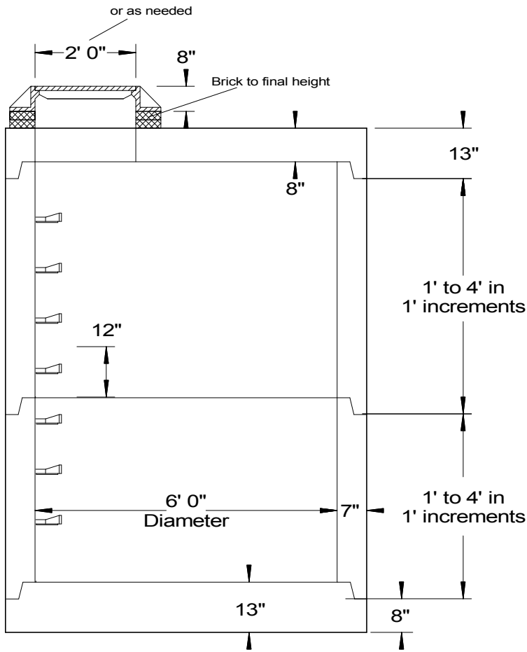
Section View
