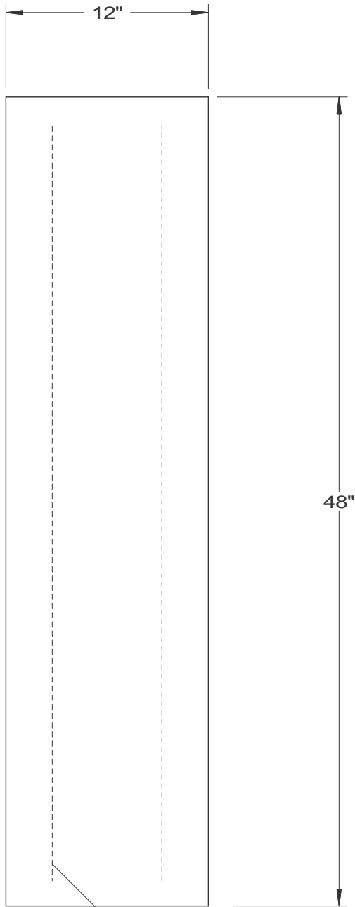
(4) 1/2" rebar
