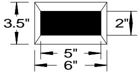
Drain Hole Detail
