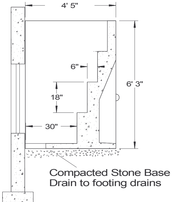
Section
