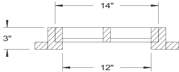
Section View
