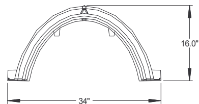
End View
